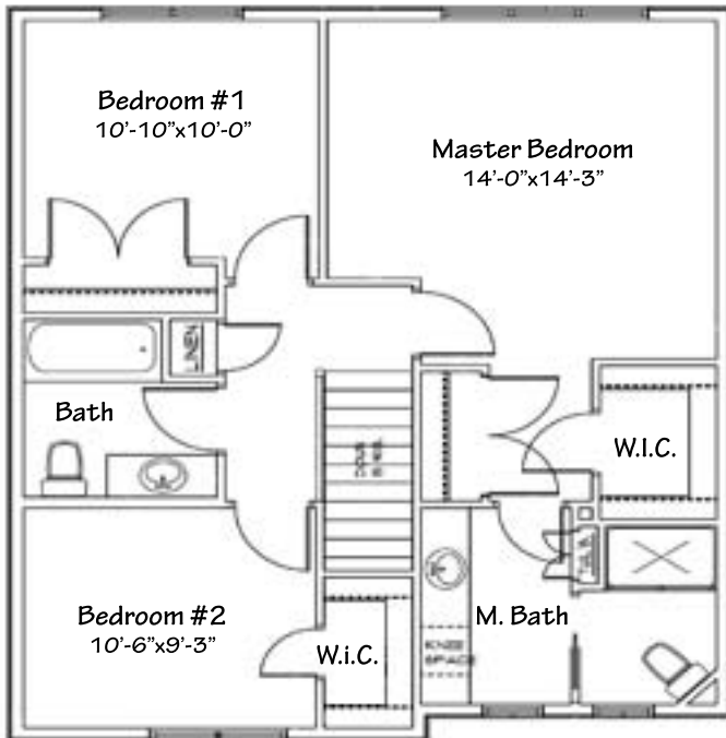
Second Floor Plan 795 Sq. Ft.
