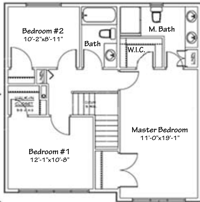
Second Floor Plan 800 Sq. Ft.
